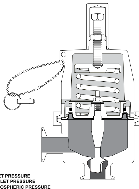
Figure 3. Type SR5 Operational Schematic
