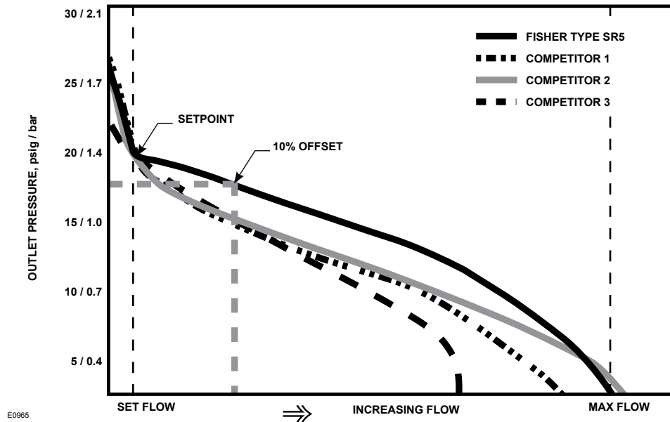
Figure 4. Type SR5 Performance Comparison
