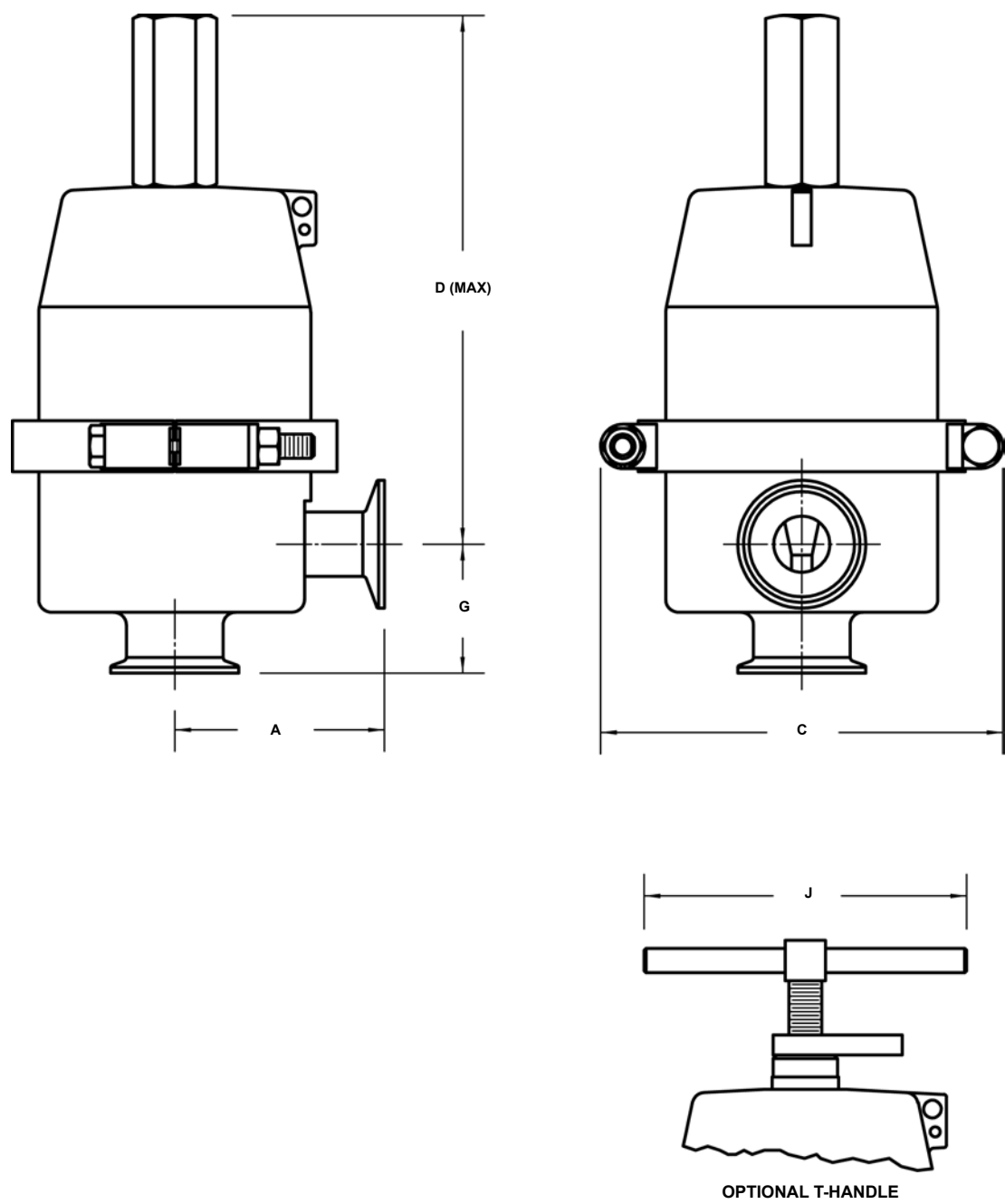
Figure 5. Dimensions
