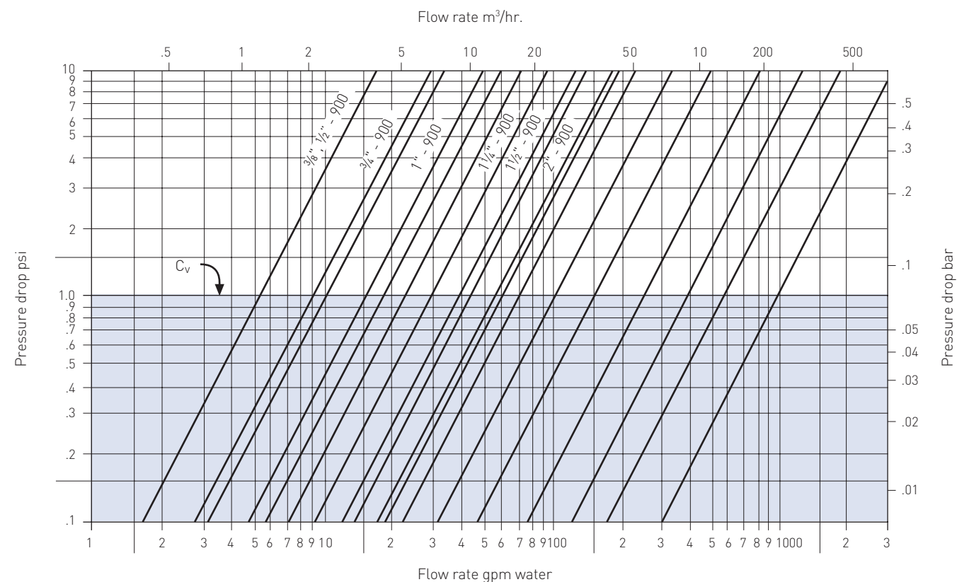
FIGURE 1 - WATER FLOW VS. PRESSURE DROP
