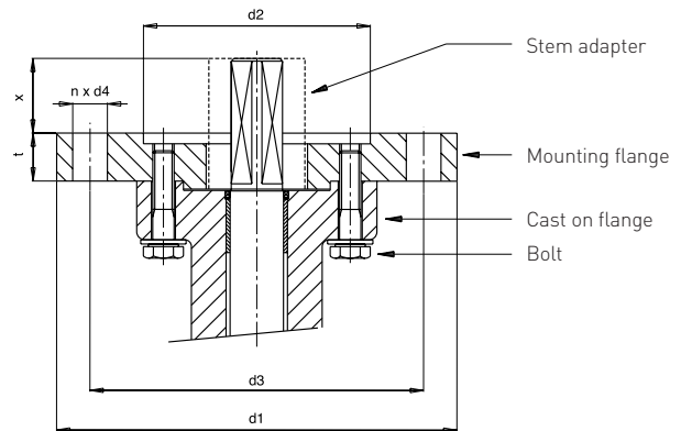
MOUNTING FLANGE
