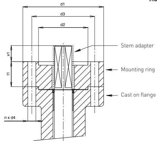
MOUNTING FLANGE
