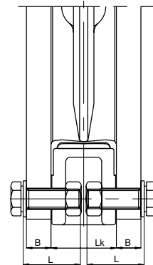
DOUBLE FLANGE
