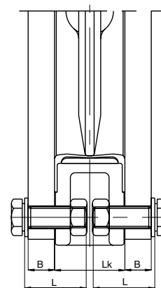
DOUBLE FLANGE
