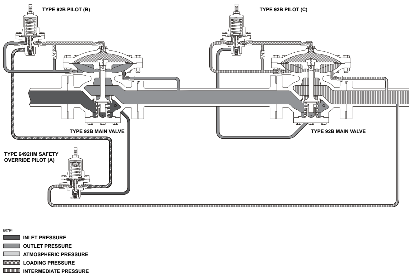
Figure 4. Safety Override System Schematic
