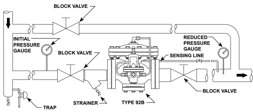
TYPE 92B SINGLE-STAGE INSTALLATION
