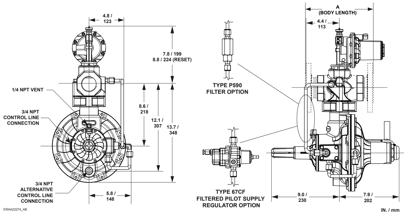
Figure 9. Types 299HS, 299HV, 299HSR and 299HVR Dimensions
