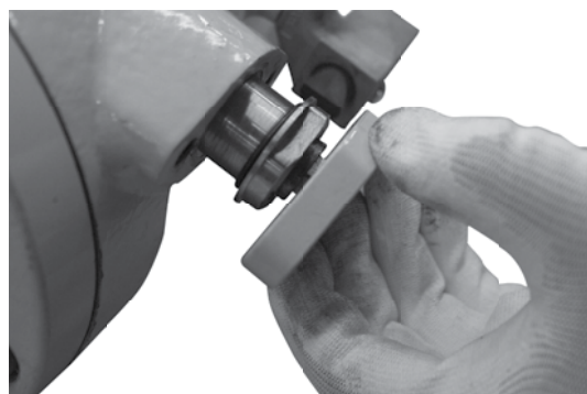
Figure 18. Install follower bearing (step 8)
