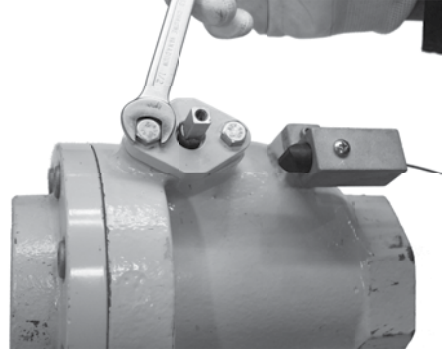
Figure 22. Wind retainer, install bolts (step 11)
