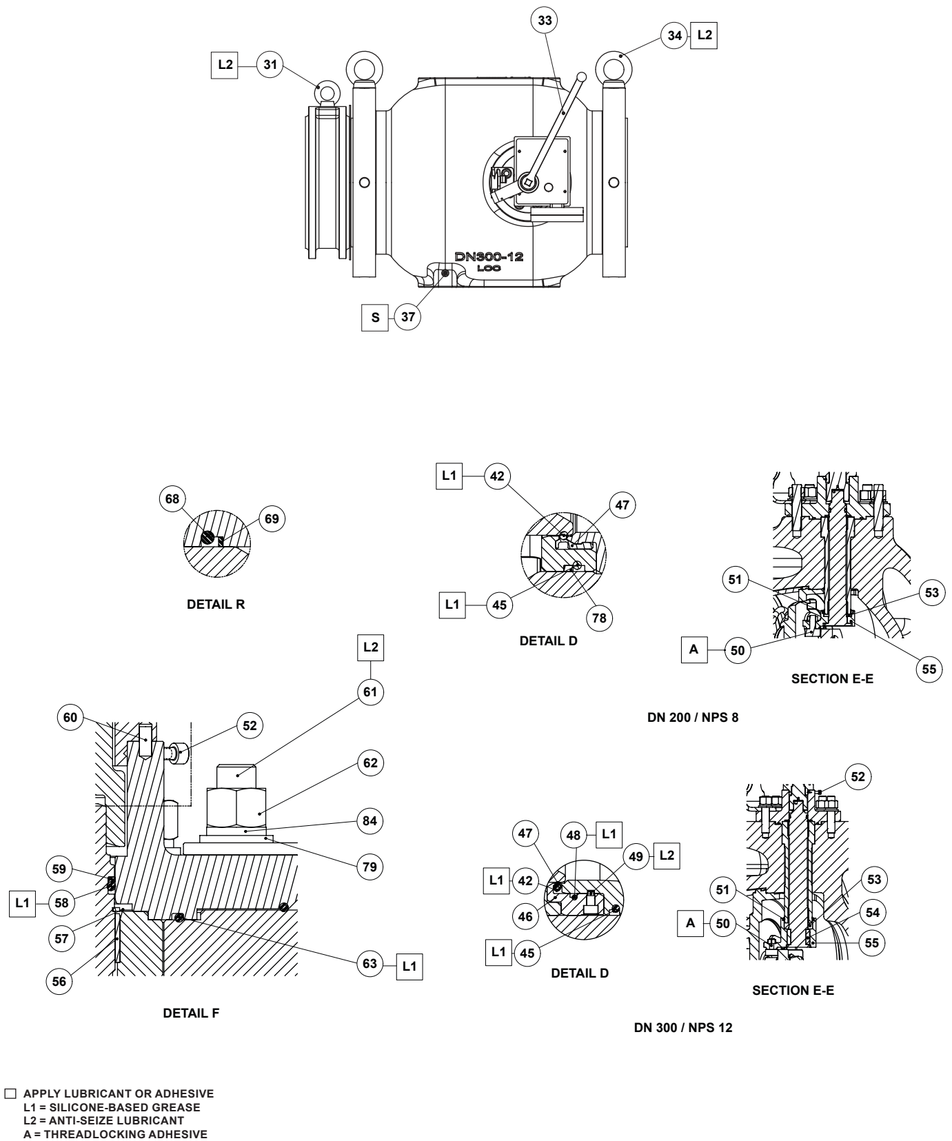
Figure 14. Type BM9 Slam-Shut Valve (continued)
