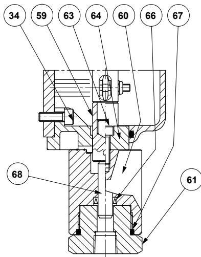
TYPE OS9/88X-R DETAIL
