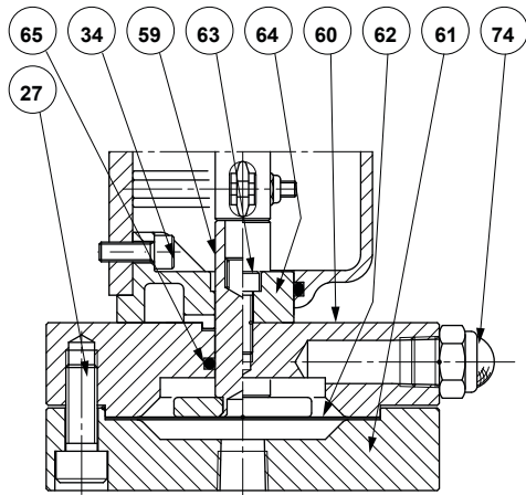
TYPE OS9/80X-APA-D-R DETAIL
