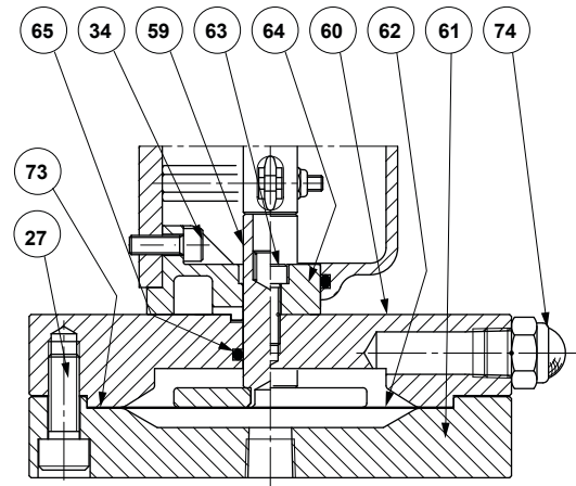
TYPE OS9/80X-MPA-D-R DETAIL
