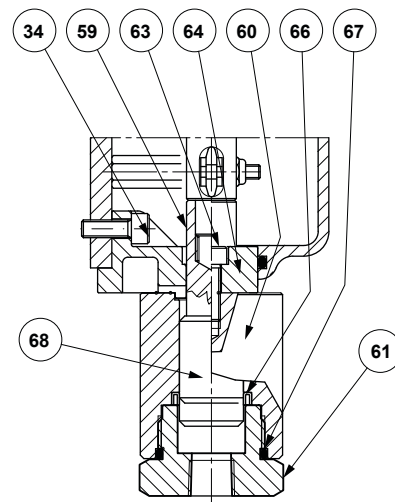
TYPE OS9/84X-R DETAIL
