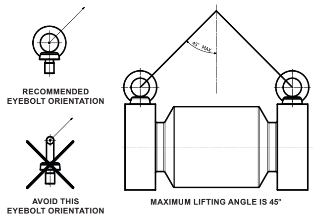
Figure 7. Lifting Lugs: Illustration of Lateral Loading
