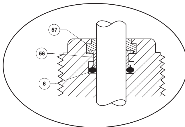
Figure 7. Type 1098 Actuator
