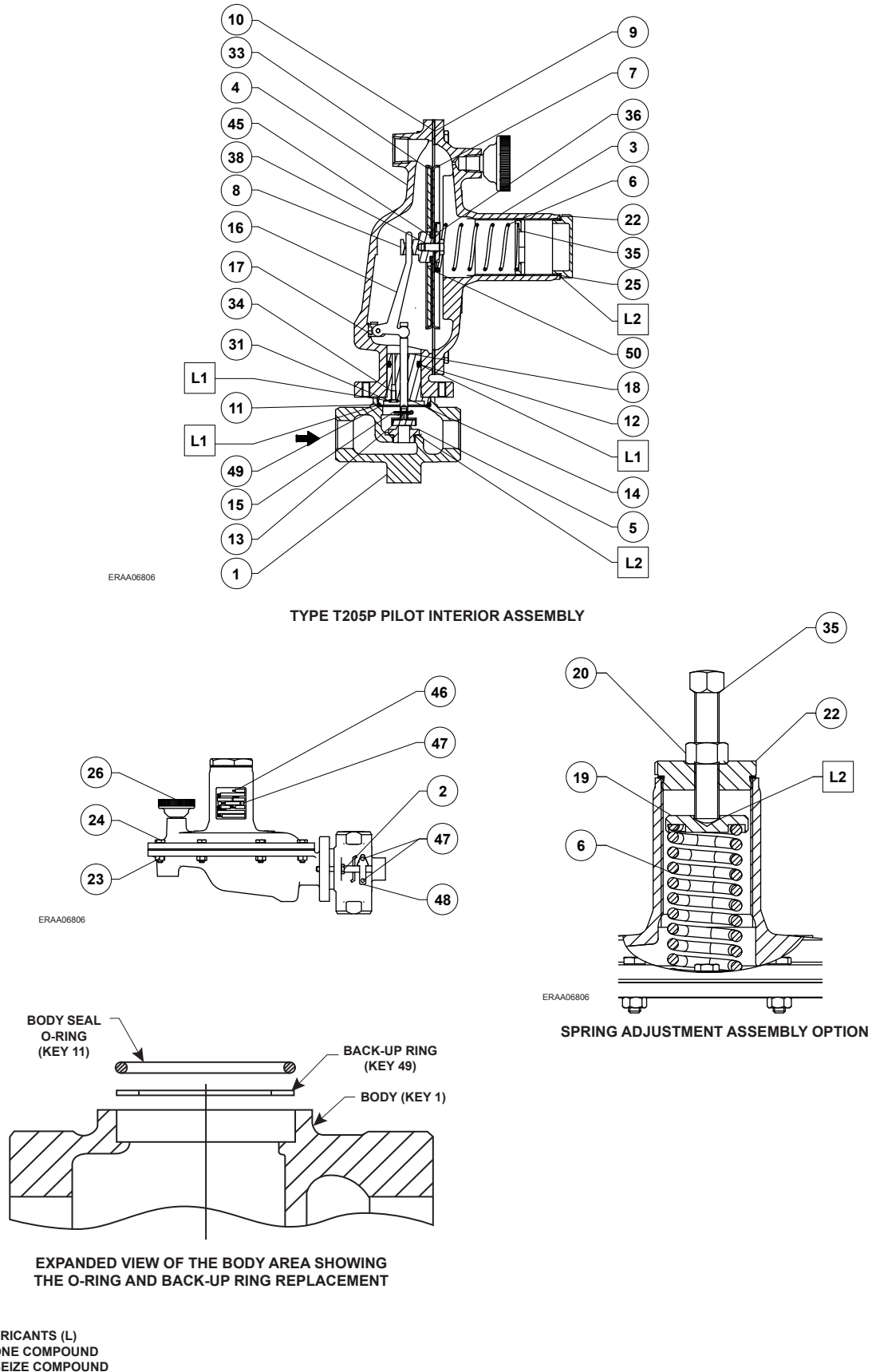
Figure 8. Type T205P Pilot Assembly Drawing
