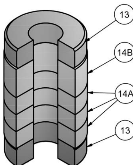
Figure 5. Molded Graphite (Flexible Graphite) Packing Kit P/N 24492T001 (Optional)
