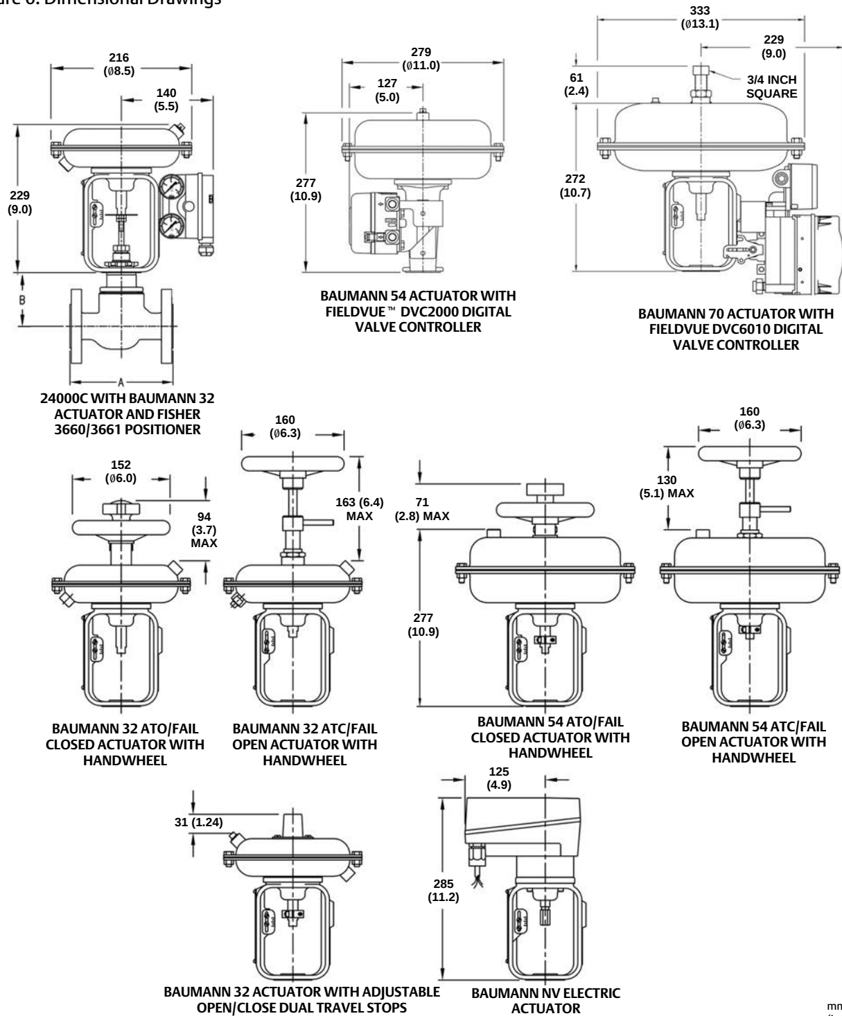
Figure 6. Dimensional Drawings
