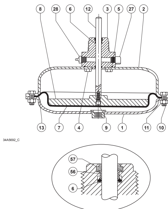
Figure 2. Type 1098 Actuator
