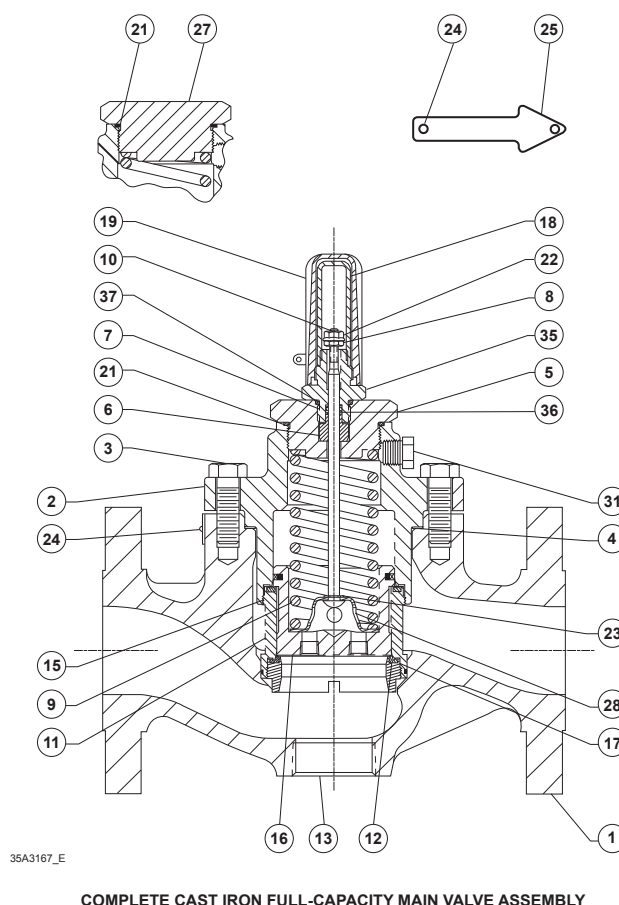
Figure 1. Type EGR Main Valve
