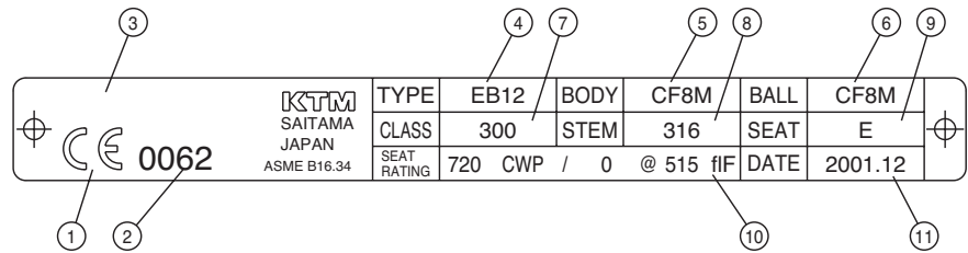
FIGURE 3 Tagplate
