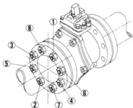
FIGURE 1 Bolting procedure
