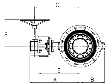
ASME B16.5 Class 600 - Trim D
