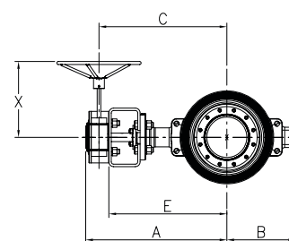
ASME B16.5 Class 150 - Trim B
