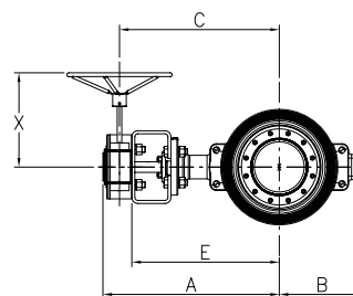
ASME B16.5 Class 600 - Trim D
