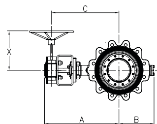
ASME B16.5 Class 600 - Trim D
