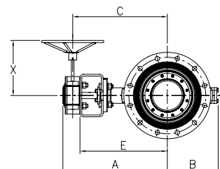
ASME B16.5 Class 600 - Trim D
