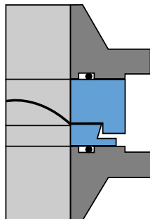
'O' ring joint for minimum leakage
