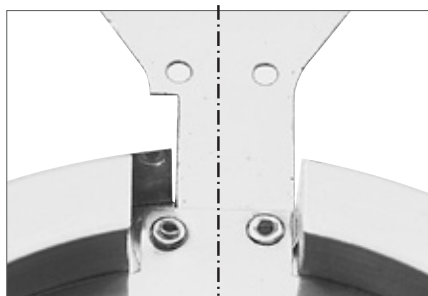
Correct assembly
