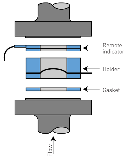
Burst disc indicator for remote fitting between holder and vent side flange.
