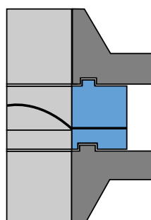
Tongue and groove
