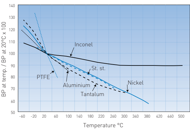
TEMPERATURE EFFECT FOR CONVENTIONAL TYPE DISCS
