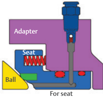
Sealant fitting with check valv embedded in shell
